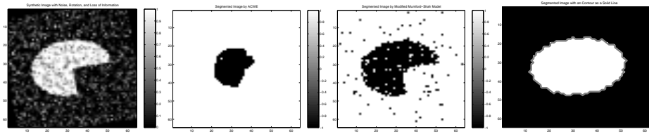
Fig. 10. First : A Given Image I , Second : Segmented Synthetic Image by an Active Contour without Edges, Third : Segmented Synthetic Image by our Proposed Model in Section 2, Fourth : Segmented Synthetic Image with a Solid Line Contour using the Prior Shape Information
