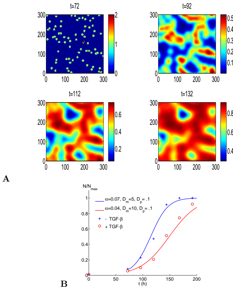
Figure 4. A Simulation of untreated cells growing according to the modified Fisher-Kolmogorov equation (3) in a square subfield of the culture dish with side 300 \mu m . Periodic boundary conditions are assumed to account for a balance of cells entering and exiting the subfield. Initially, 75 cells were seeded randomly across the domain. Snapshots are taken at t = 72 h (initial datum, upper left) and t = 92, 112 h and t = 132 h . The parameters are D_m = 5 \mu m^2 h^{-1} , D_p = 0.1 \mu m^2 h^{-1} and \alpha = 0.07 h^{-1} . B Normalised growth curves (solid curves, simulation) and experimental measurements (discrete symbols) over a time course of 5 days. Shown are the untreated cells (control, +) and cells treated with TGF-β (o).
