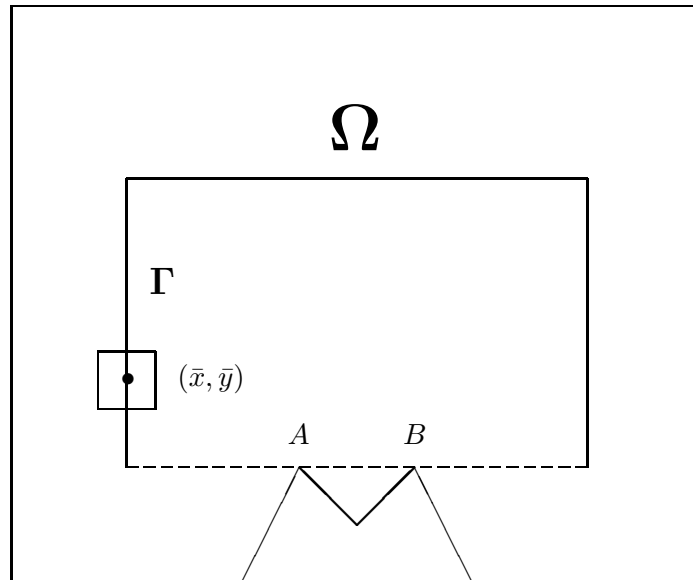
Figure 4: Paul’s limiting exit time is discontinuous at A and B . In fact, it vanishes along the segments joining A to B (and on the whole boundary), but it is bounded away from zero just above the dotted line.
