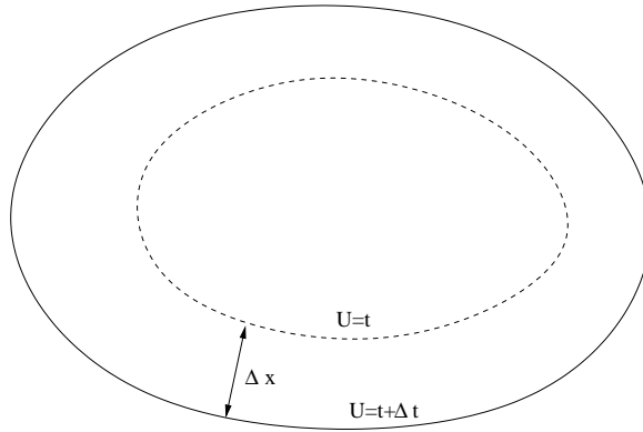
Figure 2: Level sets of U , the arrival time of the mean curvature flow.
