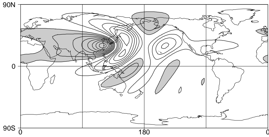
(b) Stochastic perturbation in superrotating flow
