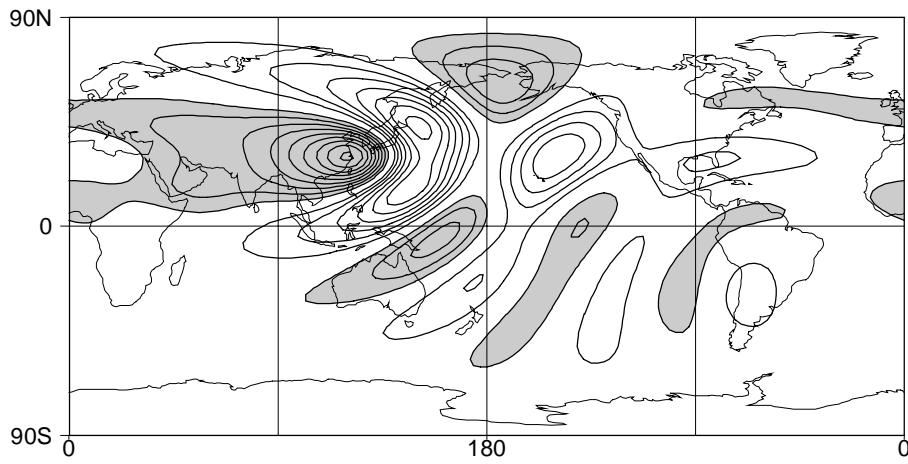
(c) Stochastic perturbation in damping
