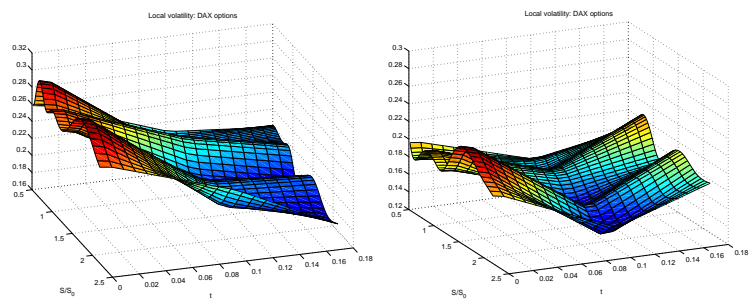
Figure 12: Local volatility surfaces: DAX options.
