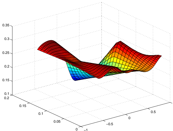
Figure 4: Local volatility function \sigma_0(\cdot, \cdot) used to generate option prices in the numerical experiments.
