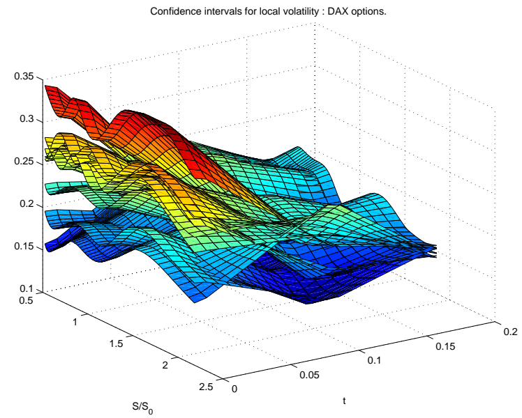
Figure 15: Uncertainty on local volatility surfaces: DAX options.
