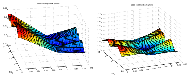
Figure 14: Local volatility surfaces: DAX options.
