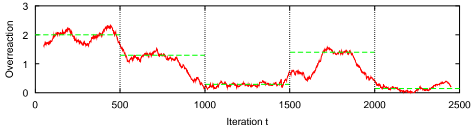
Fig. 15. Measured overreaction, i.e., difference between the actual number of decision changes (the changing rate) and the required one (the standard deviation) [117]. The overreaction can be significantly influenced by the treatment, i.e. the way of information presentation. The minimum overreaction was reached by treatment 5, i.e. user-specific recommendations.
