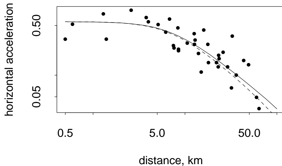
Horse Canyon, 1980 Event
