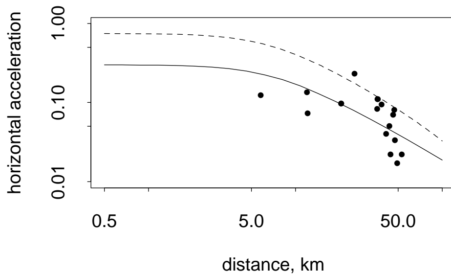
Horse Canyon, 1980 Event
